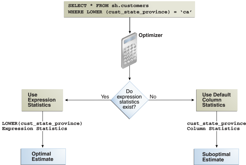
Figure 14-2 Expression Statistics
