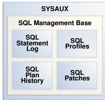
Figure 27-5 SMB Architecture
