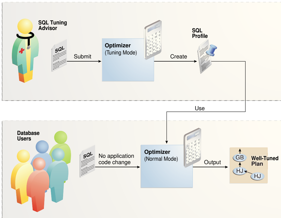
Figure 24-4 SQL Profile
