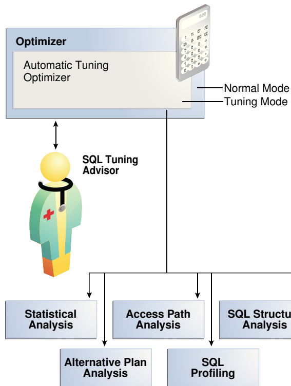
Figure 24-2 Automatic Tuning Optimizer
