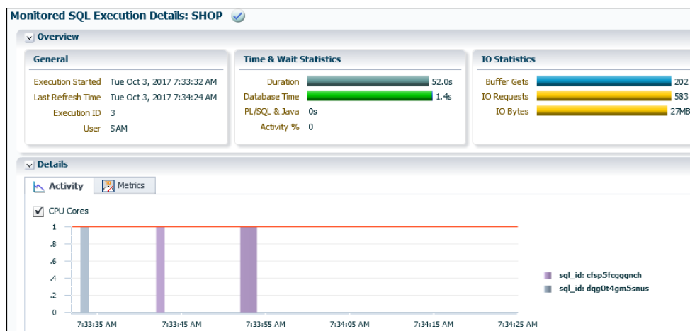
Figure 21-3 SQL Monitor Report
