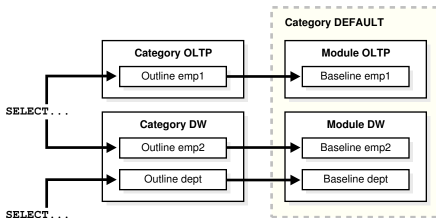
Figure 29-2 DEFAULT Category
