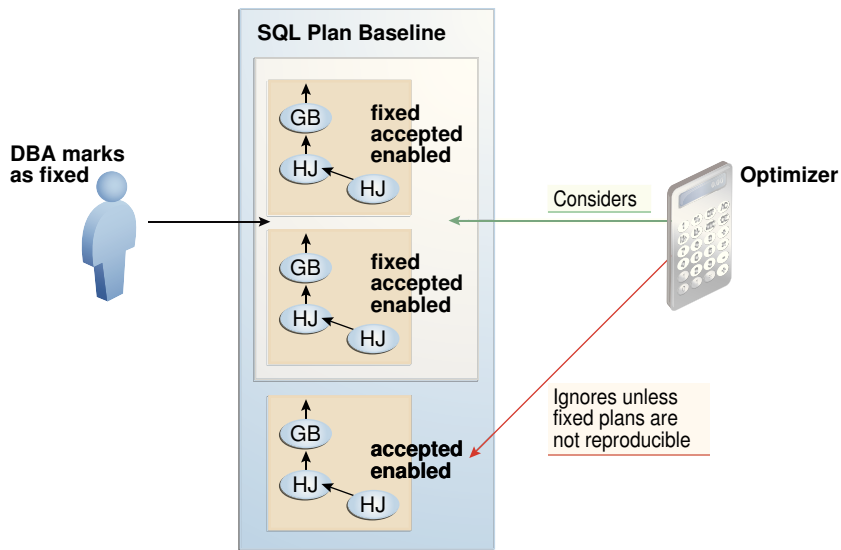
Figure 27-6 Fixed Plans
